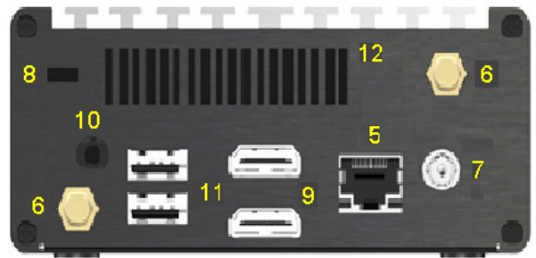
Rear I/O Port
